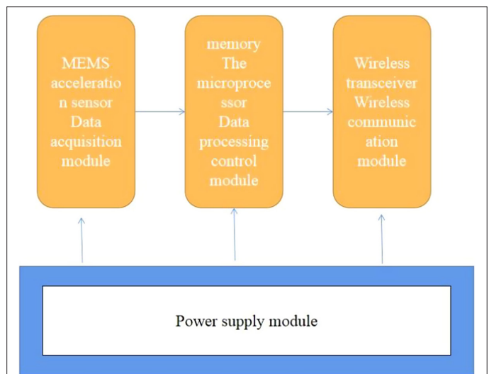
Fig. 2. Block diagram of terminal node module.
