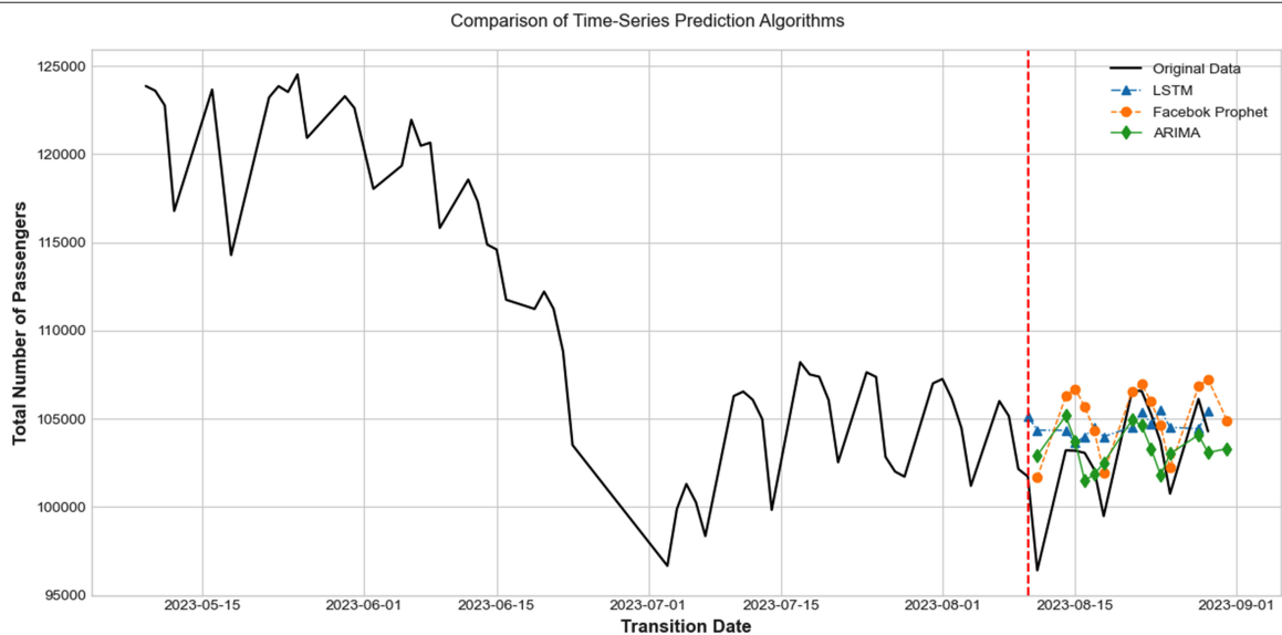
Fig. 11. Comparison of predictions LSTM, Facebook Prophet, and ARIMA. ARIMA, Autoregressive Integrated Moving Average; LSTM, long short-term memory.
