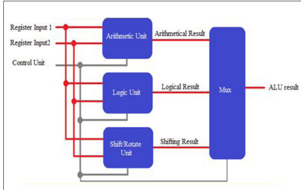
Figure 2. Arithmetic Logic Unit Design Diagram
