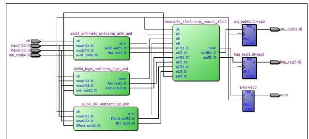
Figure 13. RTL Schema of 64 Bit Arithmetic Logic Unit
