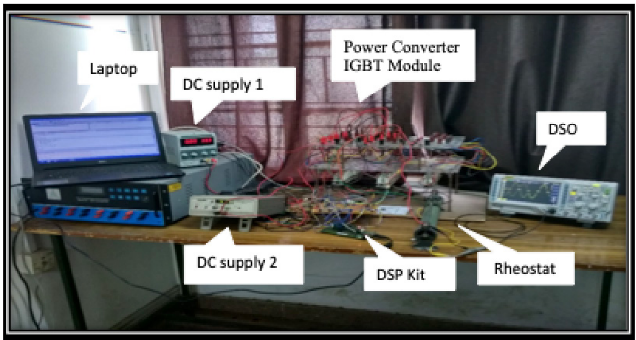
Figure 20. Experimental setup
