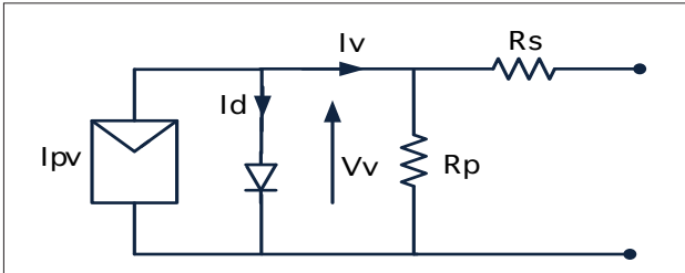
Figure 4. Single PV cell model
