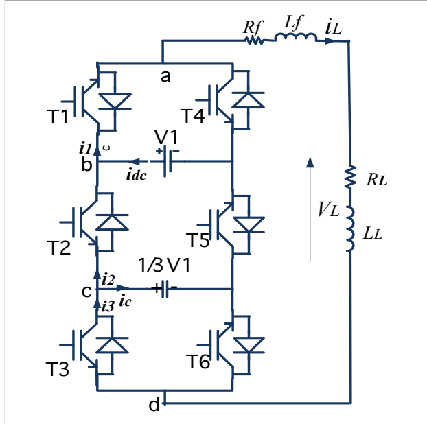
Figure 2. Packed U-Cell converter topology
