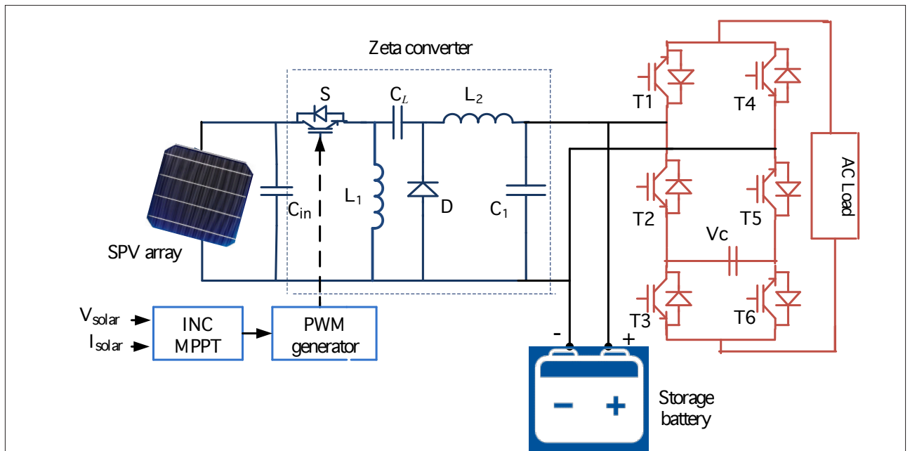
Figure 3. Proposed solar PV with zeta converter topology
