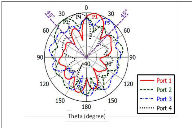
Figure 11. E-plane normalized radiation pattern of a four-element corrugated Vivaldi array fed by the Butler matrix
